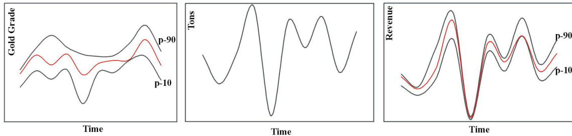
Figure 5: Geological uncertainty is the profile of possible gold grades with time (left) and production uncertainty is the profile of possible revenue forecasts (right). The transfer of geological to production uncertainty is made by multiplying grade, tons and gold price together.
