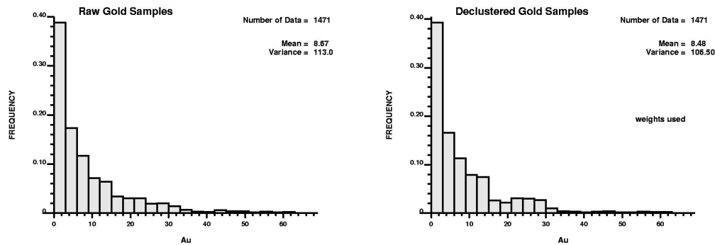
Figure 2: The raw and declustered distribution of gold grades. The declustered distribution is the target distribution and has mean and variance parameters of 8.48 and 106.50, respectively.
