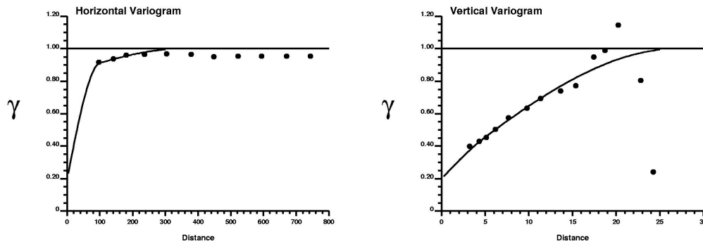
Figure 3: The horizontal and vertical gold variogram. The model variogram is shown as dark lines over top the calculated experimental points in the horizontal and vertical directions.
