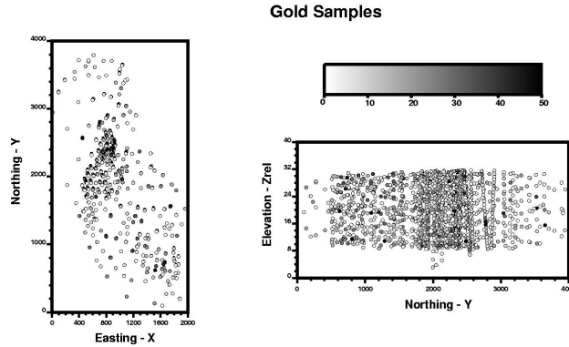
Figure 1: An X-Y plan view and Y-Zrel cross sectional view of the 1,471 gold assay locations in L1. The assays are also shaded according to gold grade.
