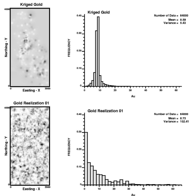
Figure 4: The distribution of gold grades is illustrated in an X-Y cross sectional view and histogram for the kriging and simulation scheme implementations.
