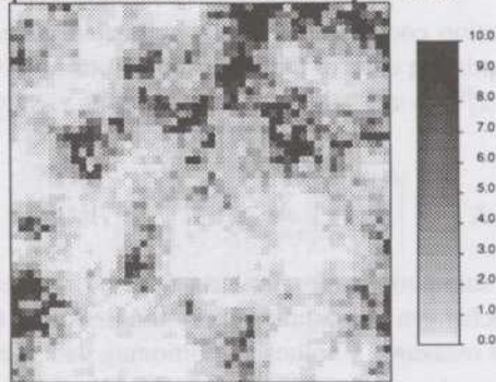
Fig. 6. A gray scale map of the truth.
