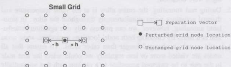
Fig. 1. An example of the two pairs that require updating after perturbing a grid node location. Only the two lags ( +\mathbf{h} and -\mathbf{h} ) require updating regardless of how large the grid network.
