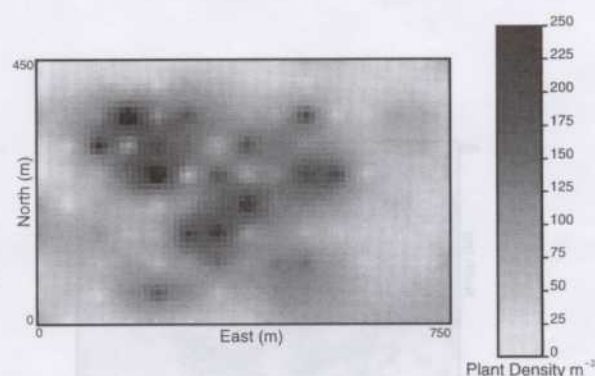
Fig. 5 A kriged map of weed density, plants m^{-2} , from the 34-ha experimental field.
