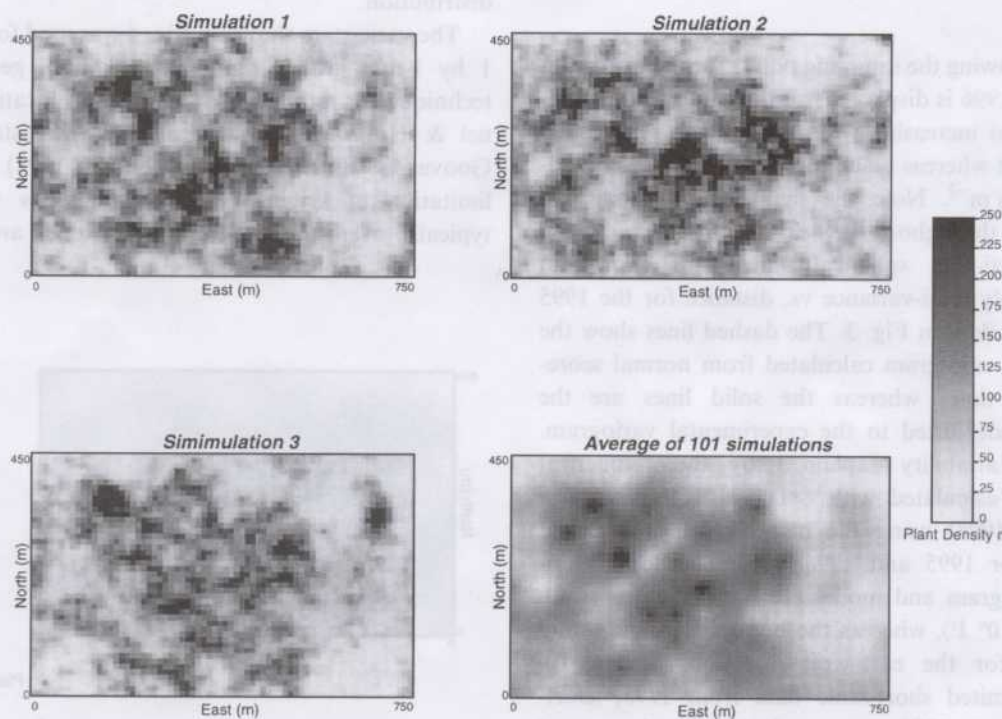
Fig. 6 Three individual simulated maps of weed density and a map of the average for 101 simulated maps of weed density (plants \text{m}^{-2} ).
