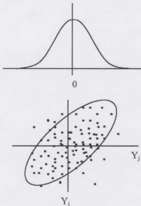
Fig. 1. Schematic illustration of a univariate and bivariate Gaussian distributions.
