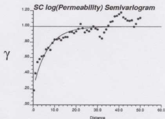
Fig. 11. Variogram of the stepwise conditional transform of permeability: used for the independent simulation of the transform of permeability.
