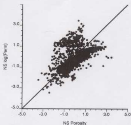
Fig. 6. Cross plot of normal score transforms of porosity and permeability. Note that these points do not follow the elliptical probability contours of the bivariate Gaussian distribution.
