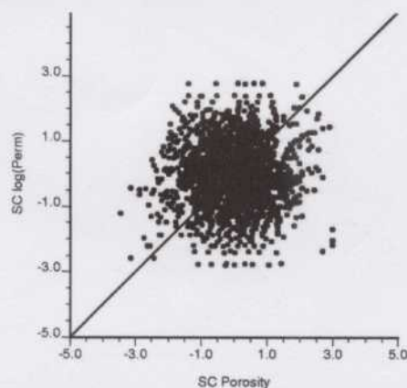
Fig. 7. Cross plot of stepwise conditional transforms of porosity and permeability. Note that these points follow a bivariate Gaussian distribution with zero correlation. There are some minor visual artifacts due to the class structure used in the transformation.
