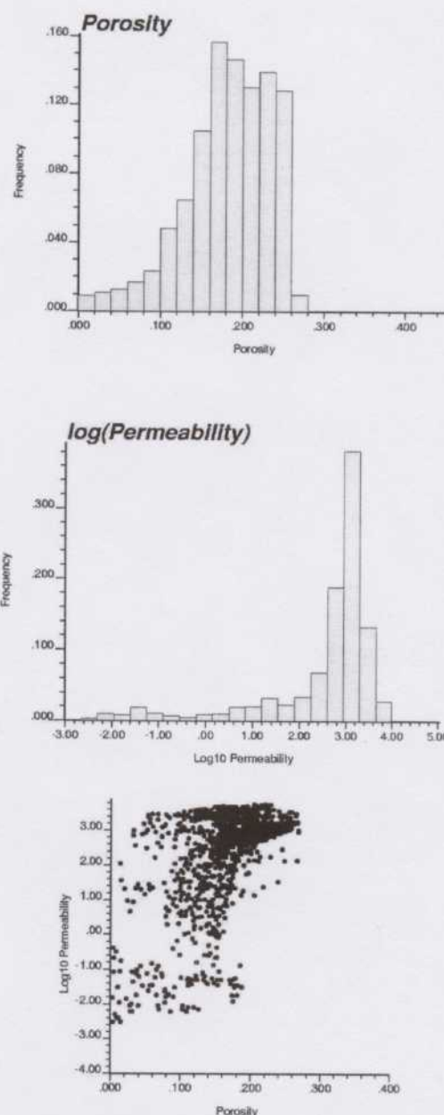
Fig. 5. Porosity / permeability data: top - porosity histogram, middle - permeability histogram, and bottom - porosity - permeability cross plot.
