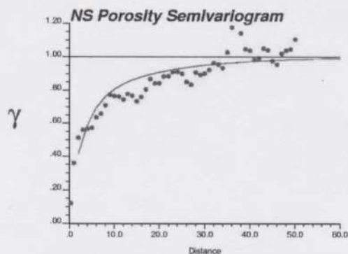
Fig. 8. Variogram of the normal score transform of porosity. This variogram is used for the simulation of porosity in both the conventional and the stepwise approach.
