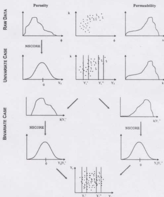
Fig. 4. Illustration of stepwise conditional transformation for two-variables (porosity and permeability). The top row of the Figure shows the porosity histogram, porosity-permeability cross plot, and permeability histogram. The second row from the top labeled Univariate Case shows the normal score transform of porosity; the permeability is left unchanged, but the central cross plot changes because the porosity has been transformed to normal space. The third and fourth rows from the top labeled Bivariate Case shows how the permeability values are transformed according to conditional distributions given the porosity values. The left side shows the transformation of permeability values belonging to a "low" class of porosity; the right side shows transformation of permeability values belonging to a "high" class of porosity.
