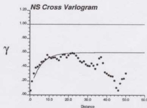
Fig. 10. Cross variogram between the normal score transform of porosity and the normal score transform of permeability. This variogram would only be used for a full cosimulation approach. In practice the collocated cosimulation approach is used and this variogram is never explicitly used in reservoir modeling.
