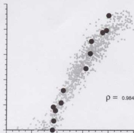
Fig. 18. Twelve hard data (large black dots) and modeled data to permit reliable inference of conditional distributions.
