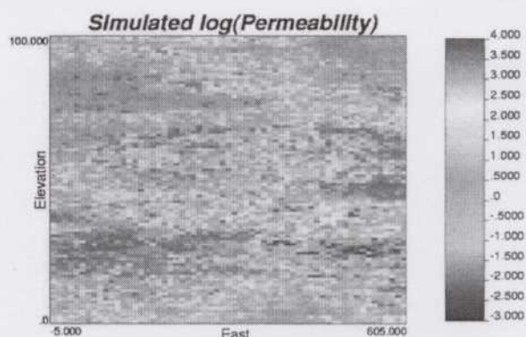
Fig. 14. Color scale image (in log scale) of simulated permeability from stepwise approach, that is, independent simulation of the stepwise conditional transform and then back transform according to correct conditional distributions.
