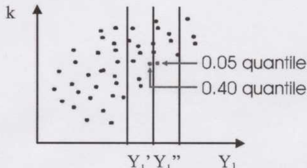
Fig. 17. Schematic illustration showing how two data points of essentially the same values can lead to different transformed values if the number of classes and data are too few.
