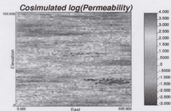
Fig. 13. Color scale image (in log scale) of simulated permeability using collocated cosimulation with correlation coefficient of 0.59. Note the correlation with porosity on Fig. 12.
