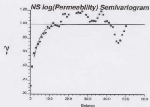
Fig. 9. Variogram of the normal score transform of permeability. This variogram is only used for the simulation of permeability in the conventional approach.
