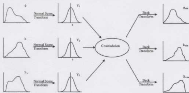
Fig. 3. Procedure for conventional Gaussian simulation for reservoir modeling: the original data are normal score transformed to normal variables, these variables are cosimulated accounting for correlation, and then back transformed to the correct units.
