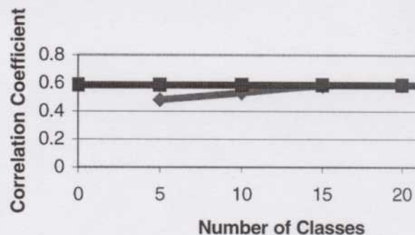
Fig. 16. Convergence of the correlation coefficient with increasing number of classes in the stepwise conditional transformation procedure.
