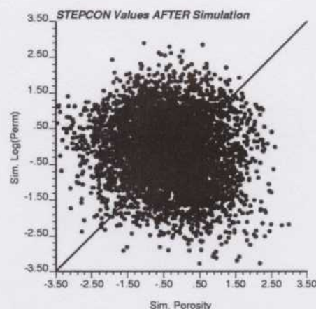
Fig. 15. The "normal-space" cross plots between porosity and permeability. In the top case (conventional) the relation is bivariate Gaussian with the correct correlation coefficient, but does not have the same features as Fig. 6. The lower cross plot shows a bivariate Gaussian relation with no correlation, which is required by the stepwise conditional approach.
