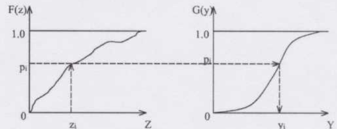
Fig. 2. Illustration of normal score transform. The cumulative probability p_i of the original data z_i is determined, then the matching normal value y_i is calculated.
