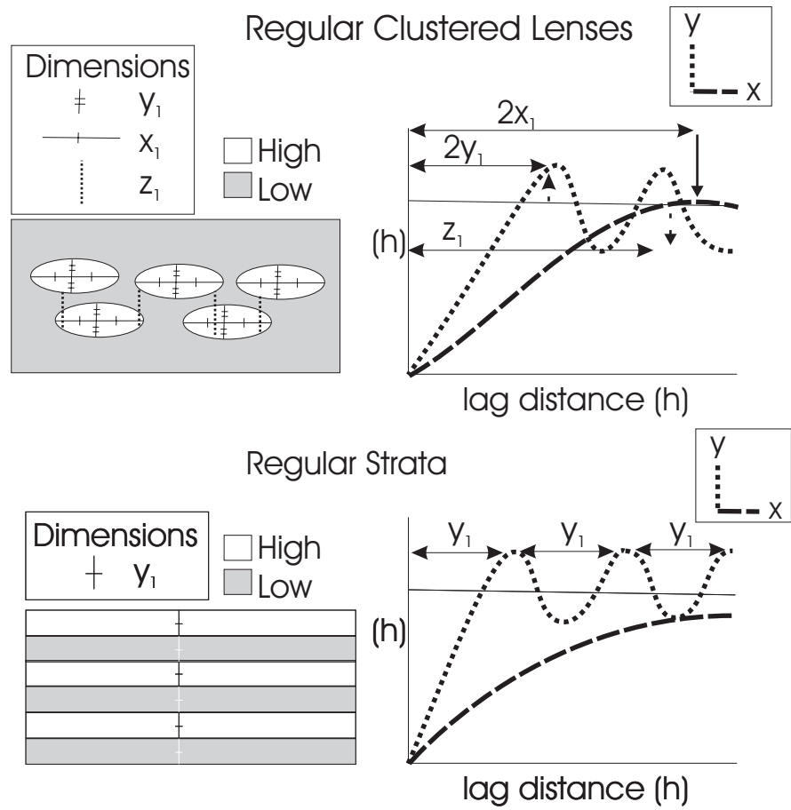
Figure 3: Hole effect interpretations in regular clustered lenses and regular strata based on indicator data
