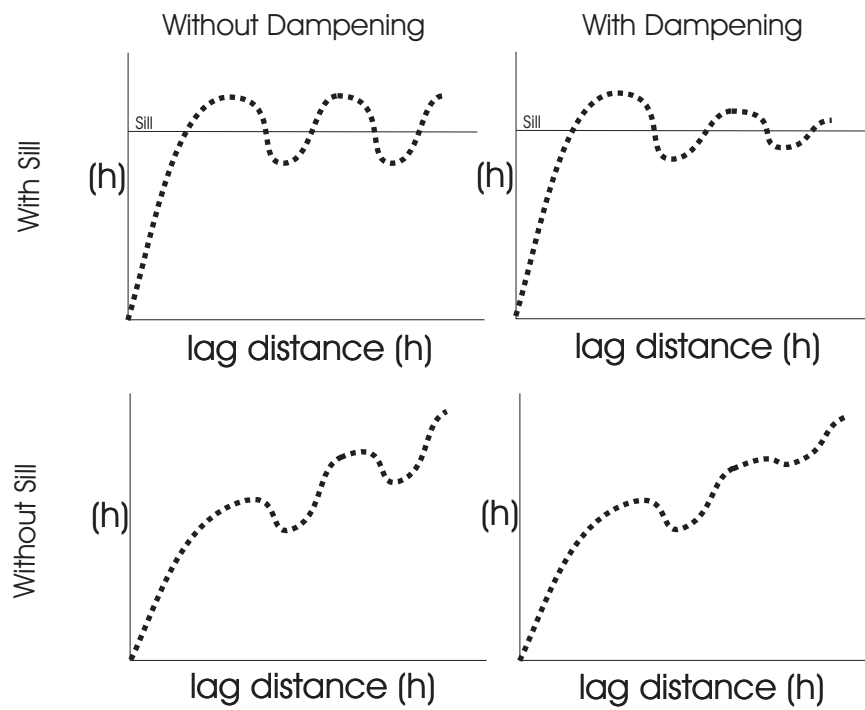
Figure 2: Hole effect configurations: The observed cyclicity may be dampened. In this case the amplitude is reduced with each subsequent wavelength. The variogram may be bounded by a sill occur without a sill.
